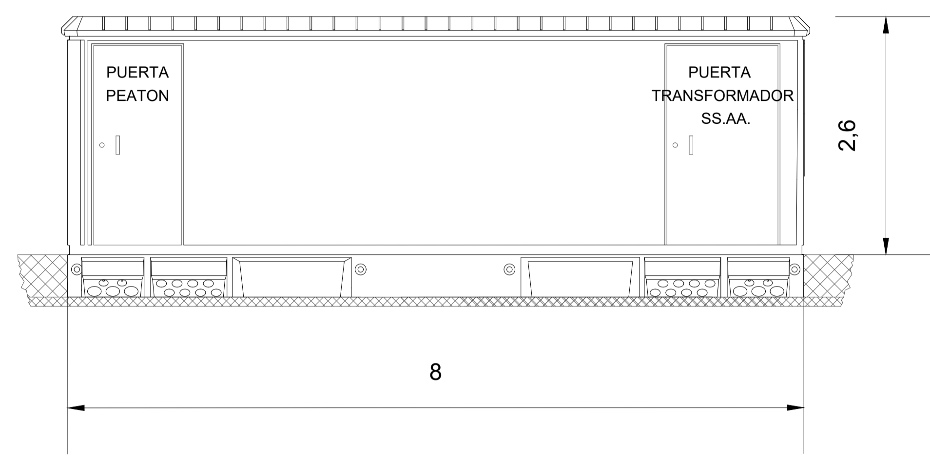
VISTA FRONTAL
