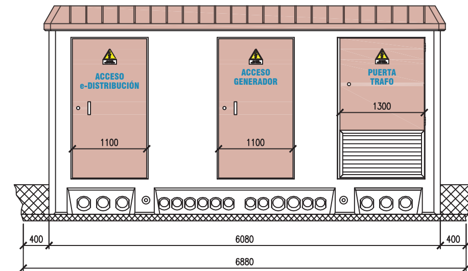
VISTA FRONTAL
