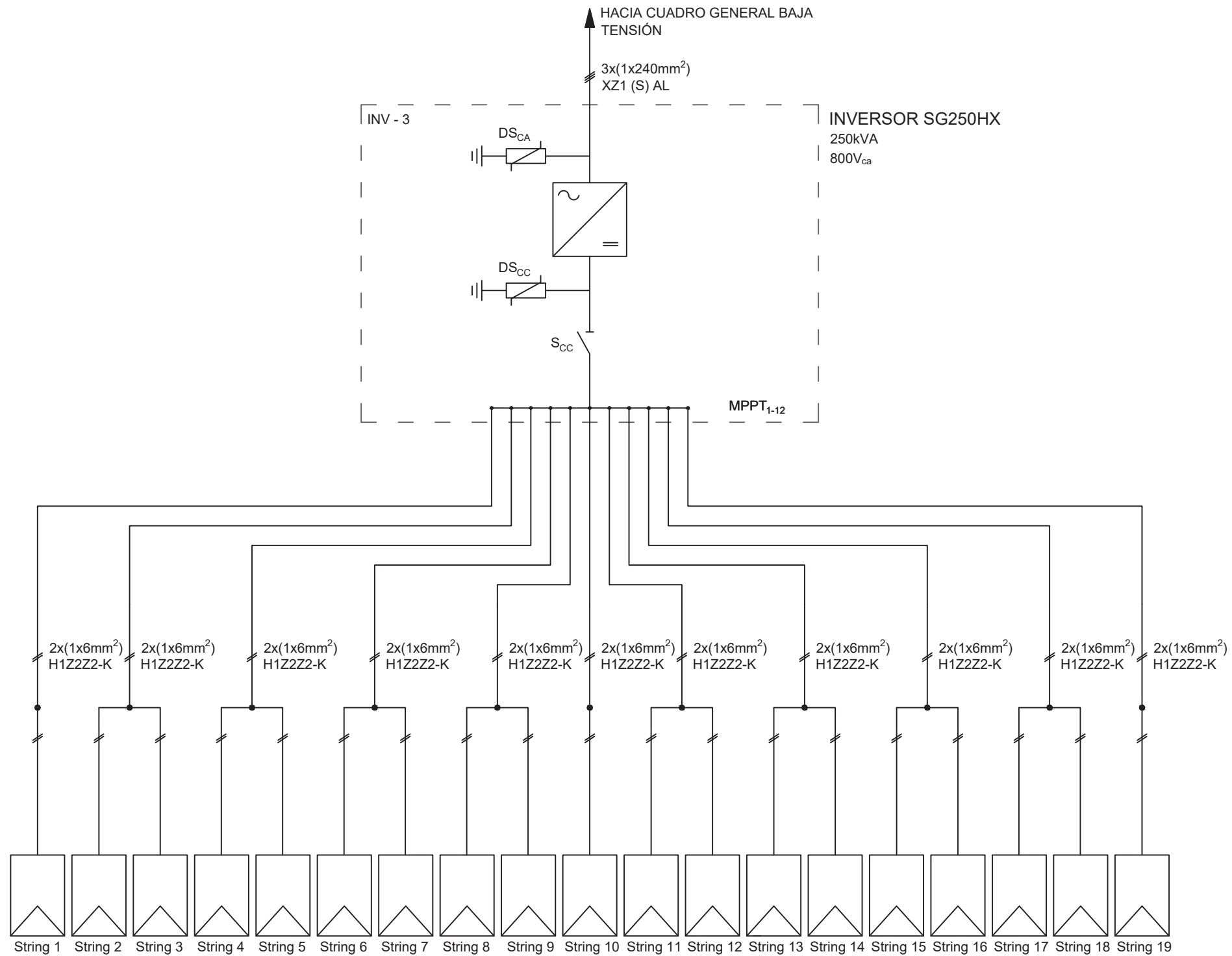
INVERSOR SG250HX
