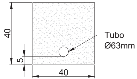
ZANJA STRING-1
