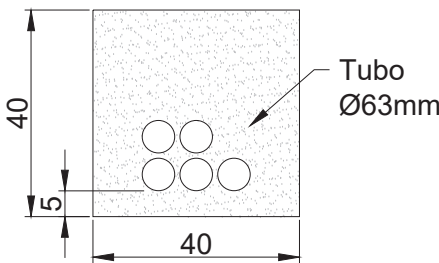
ZANJA STRING-5
