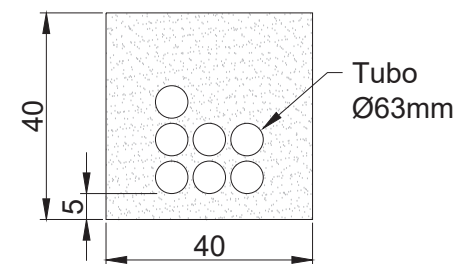
ZANJA STRING-7
