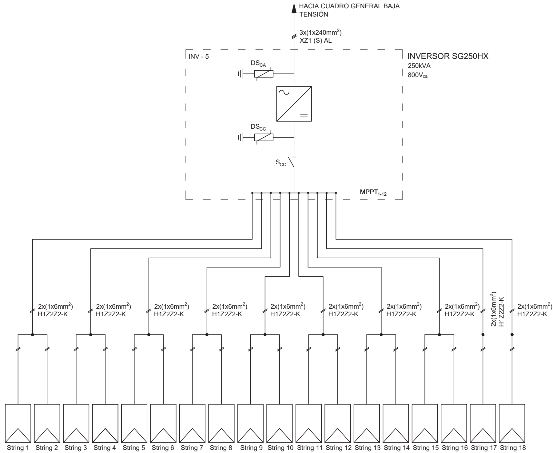
INVERSOR SG250HX
