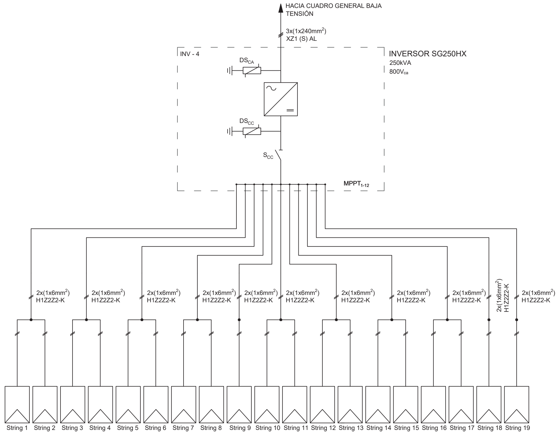
INVERSOR SG250HX
