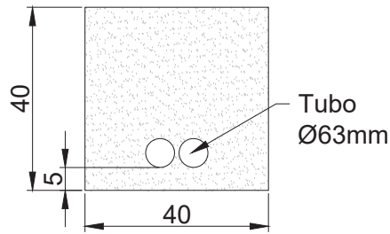
ZANJA STRING-2
