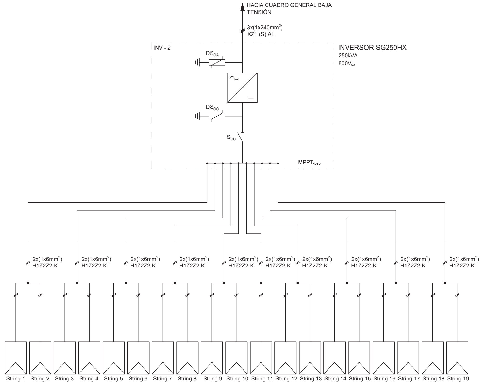
INVERSOR SG250HX
