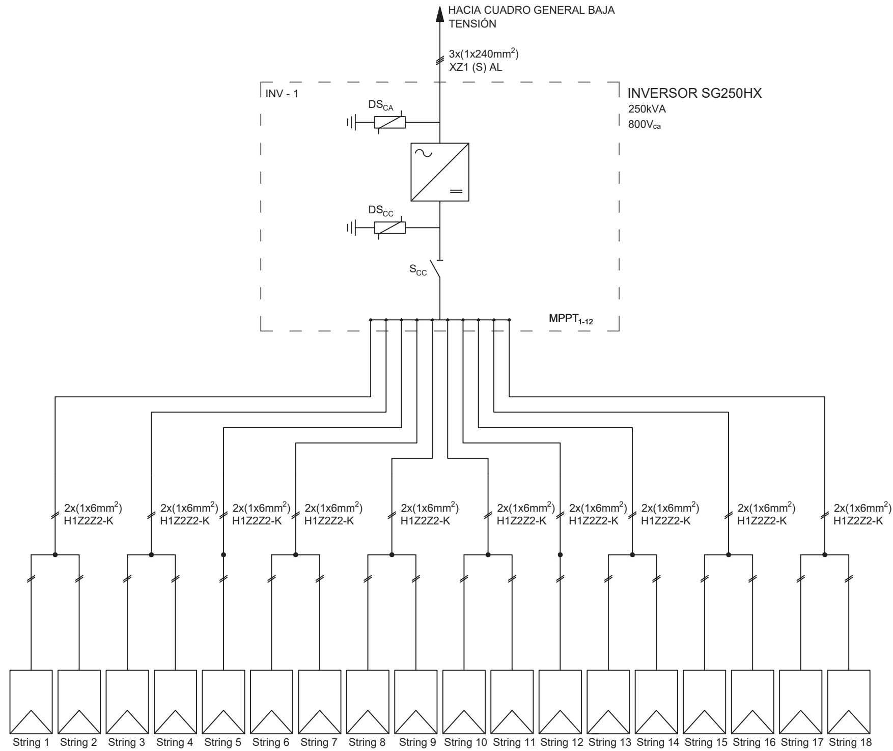
INVERSOR SG250HX
