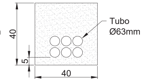
ZANJA STRING-6
