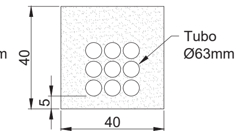
ZANJA STRING-9
