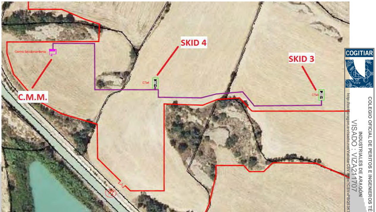
Detalle Circuito 2 "Skid 3 – Skid 4 – CMM"
