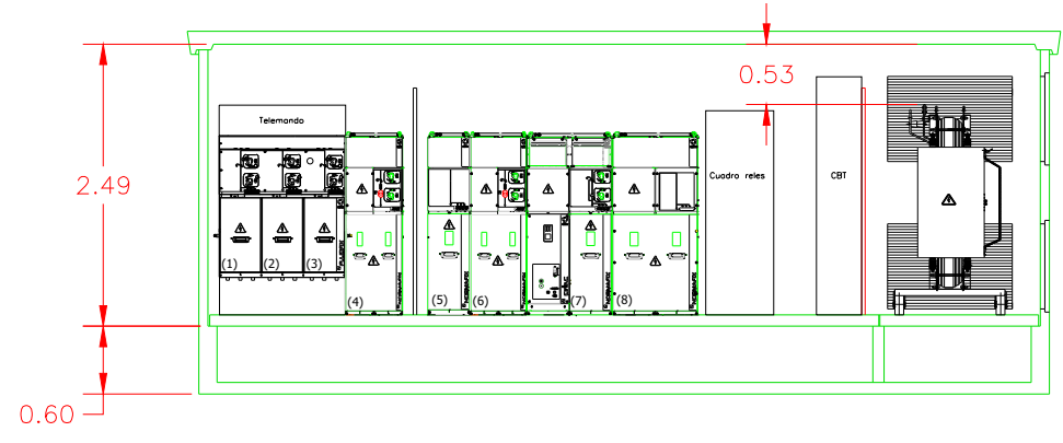
ALZADO PRINCIPAL
