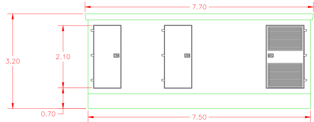
ALZADO PRINCIPAL
